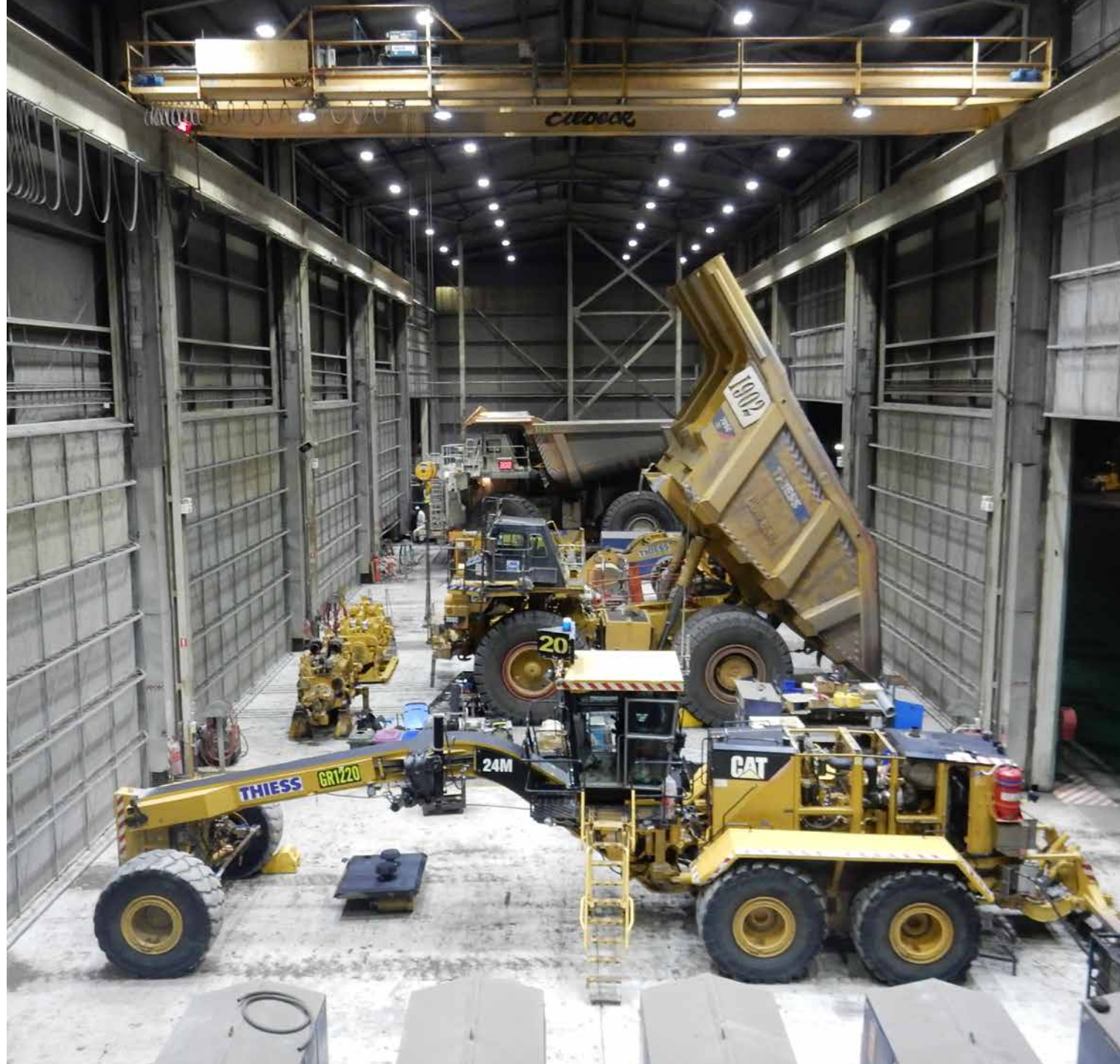
GLENCORE, MOUNT OWEN - HEAVY VEHICLE WORKSHOP 40 x 320W Mega floods in 415VAC with 60 degree lenses, delivering 600 lux average.
